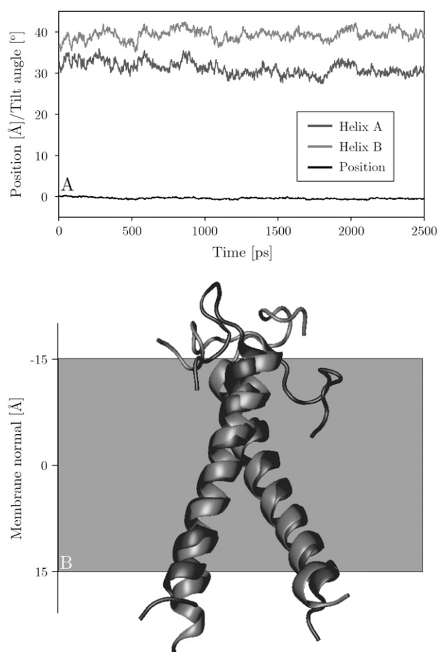
FIGURE 7 (A) Tilt angles of helices A and B, and center of mass position of the glycoporphin A dimer simulation. (B) Initial global minimum energy configuration of the glycoporphin A dimer TM domain (1afo, model 12) in black. The final structure at the end of the simulation (2.5 ns) is shown in gray. This model is representative of the 11 of 20 structures that were found to insert.
